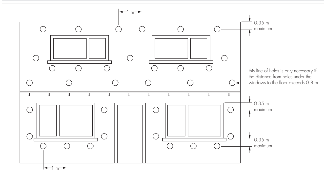
Figure 1 Typical drilling pattern — frontage
