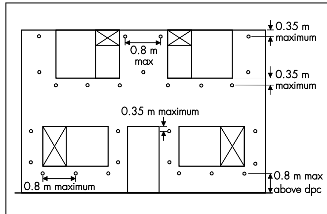
Figure 1 Typical drilling pattern — frontage
