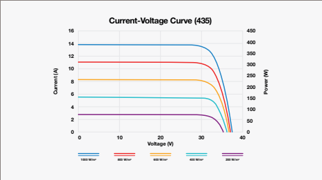
IV CURVE
